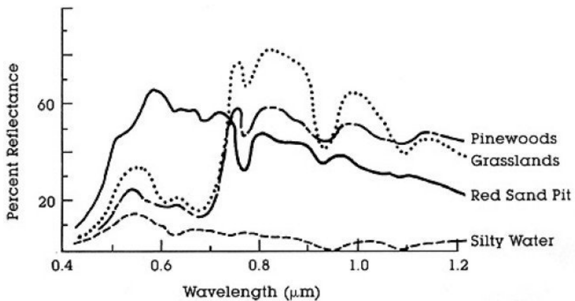
Fig. 13.2: Spectral Reflectance Curves of Four Different Targets (from NASA, 2013)
