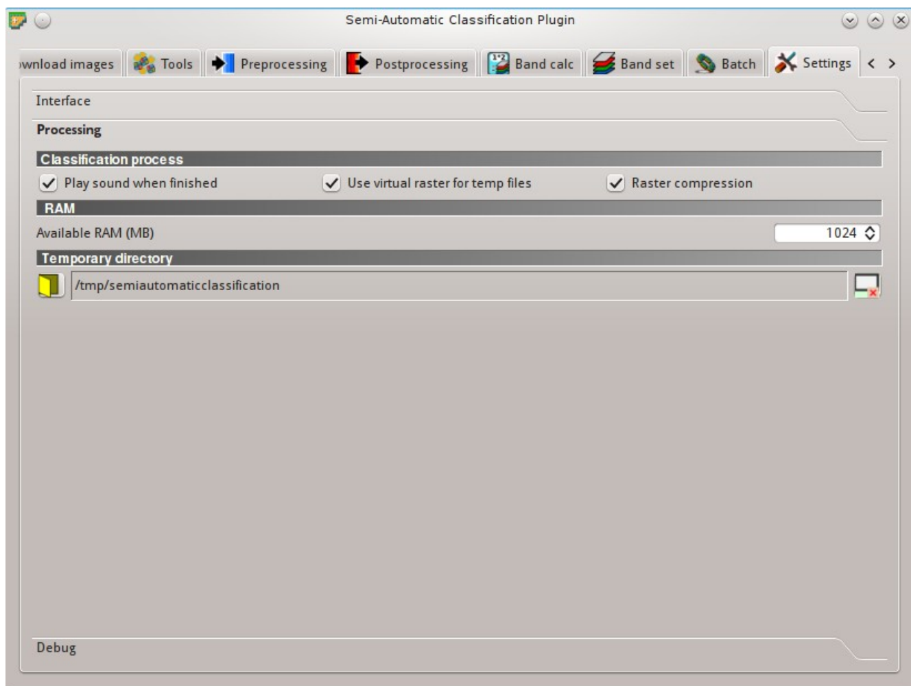
Fig. 10.35: Processing
