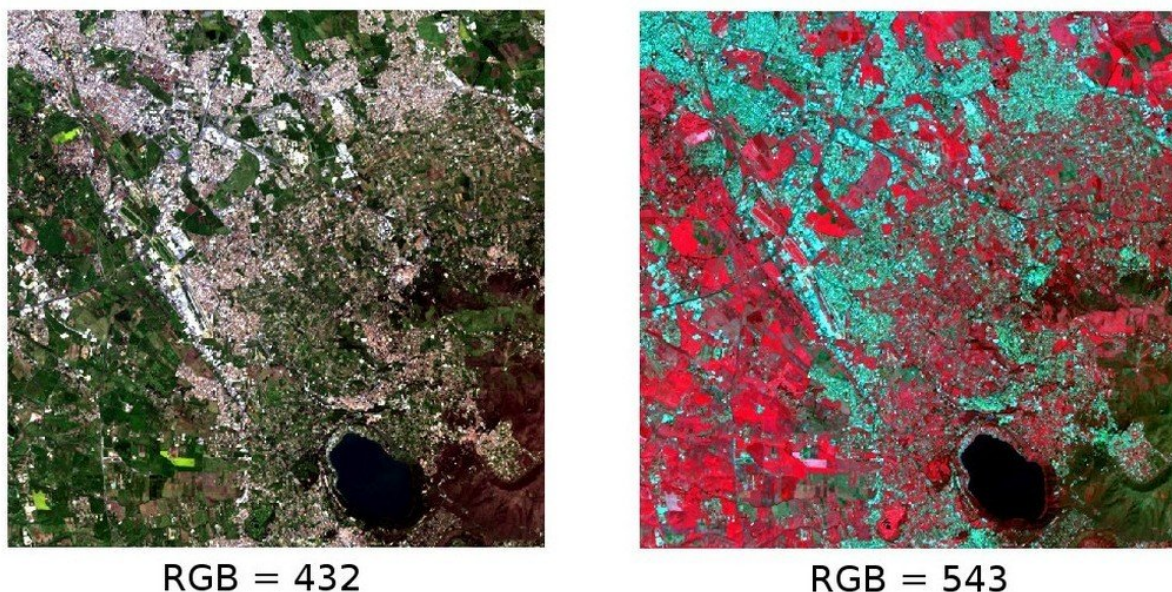
Fig. 13.3: Color composite of a Landsat 8 image Data available from the U.S. Geological Survey
