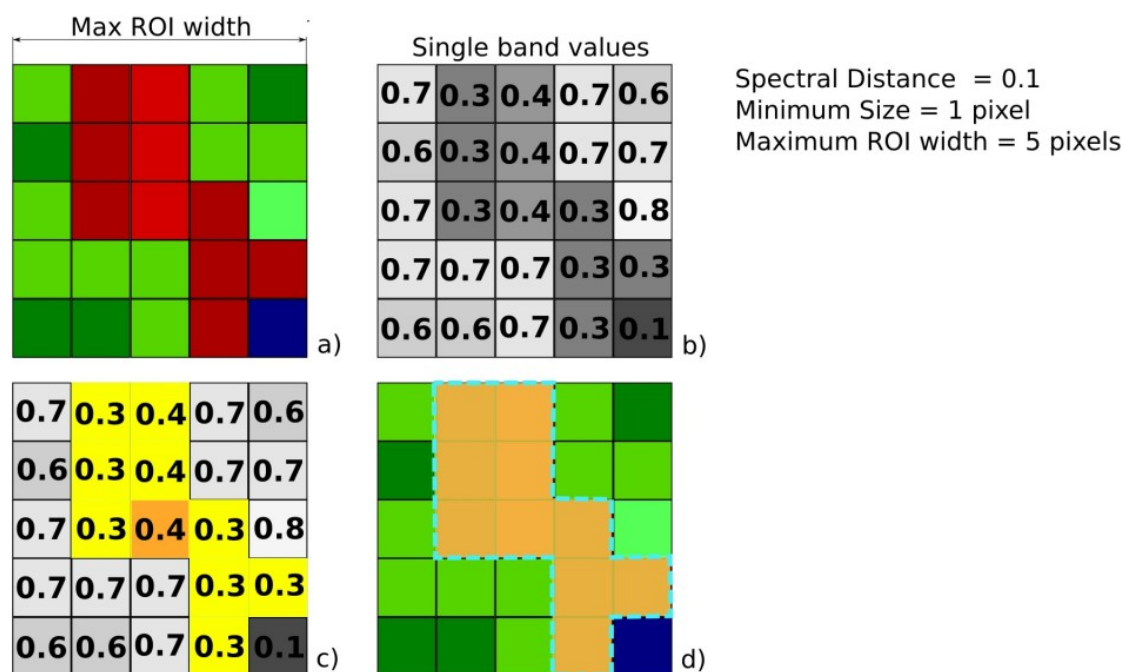
Fig. 14.2: Region growing example
