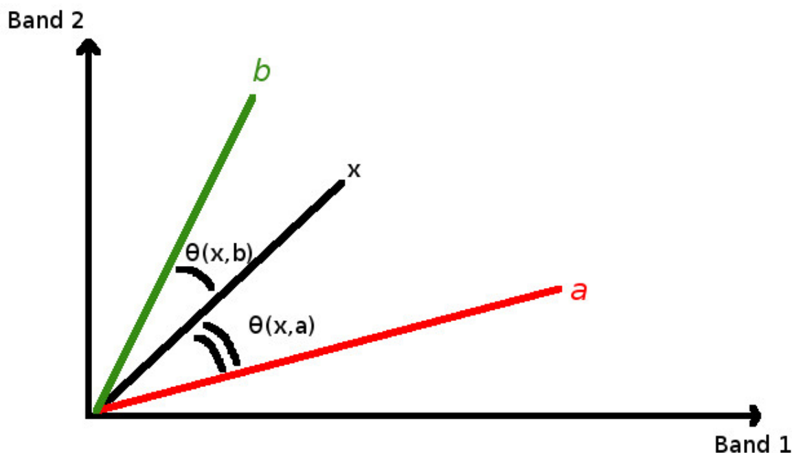
Fig. 14.5: Spectral Angle Mapping example
