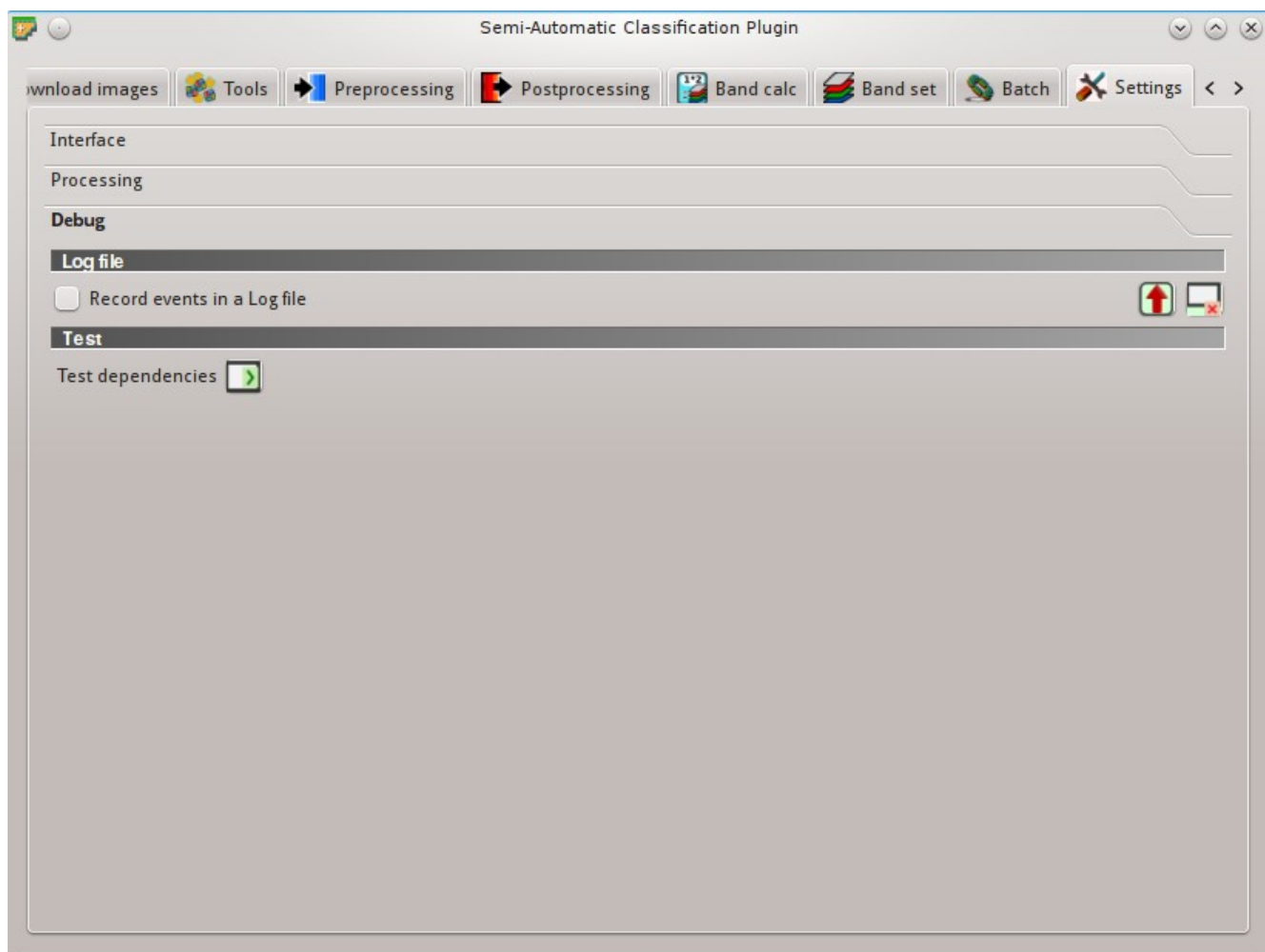
Fig. 10.36: Debug
