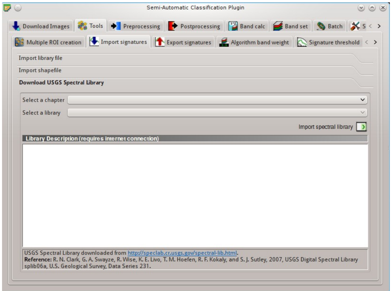
Fig. 10.9: Download USGS Spectral Library
