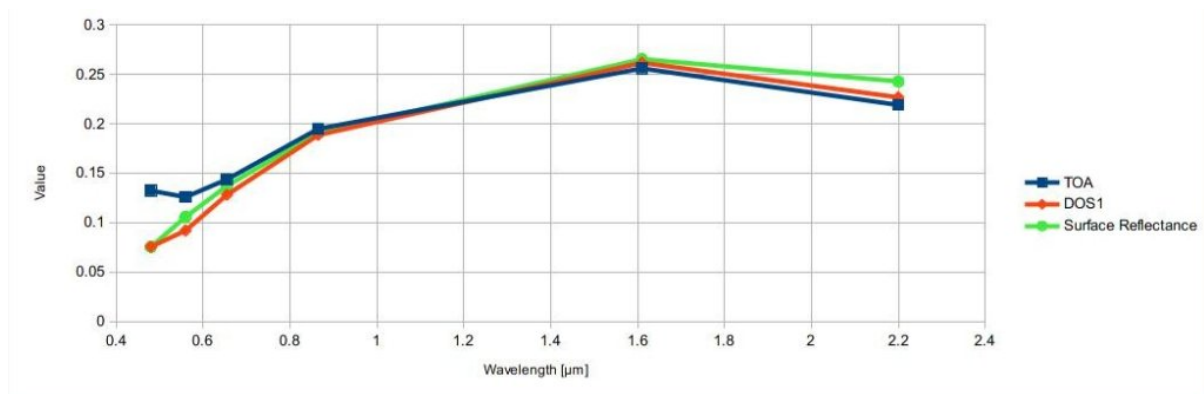
Fig. 15.1: Spectral signatures of a built-up pixel
