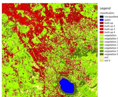
Fig. 14.8: Landsat classification
