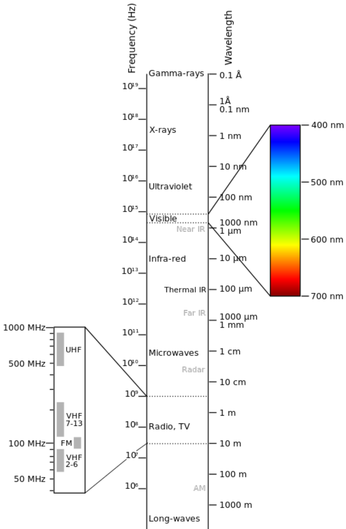
Fig. 13.1: Electromagnetic-Spectrum
